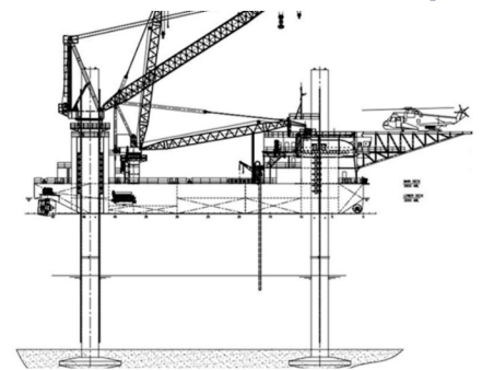
Lift Boat
